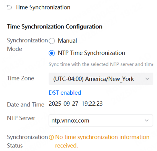
Figure 7-20 NTP Time Synchronization
