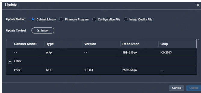
Figure 7-44 Update cabinets
