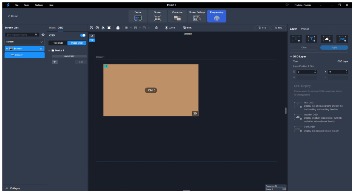
Figure 7-37 Enable OSD
