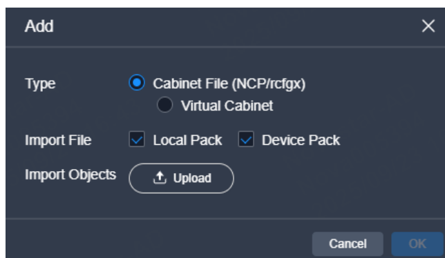
Figure 7-46 Cabinet files
