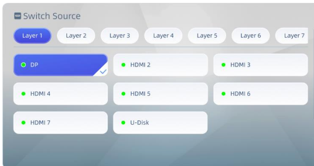
Figure 6-4 Interface example
