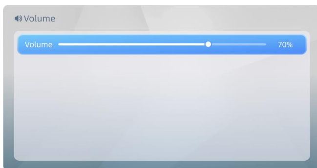
Figure 6-9 Screen example
