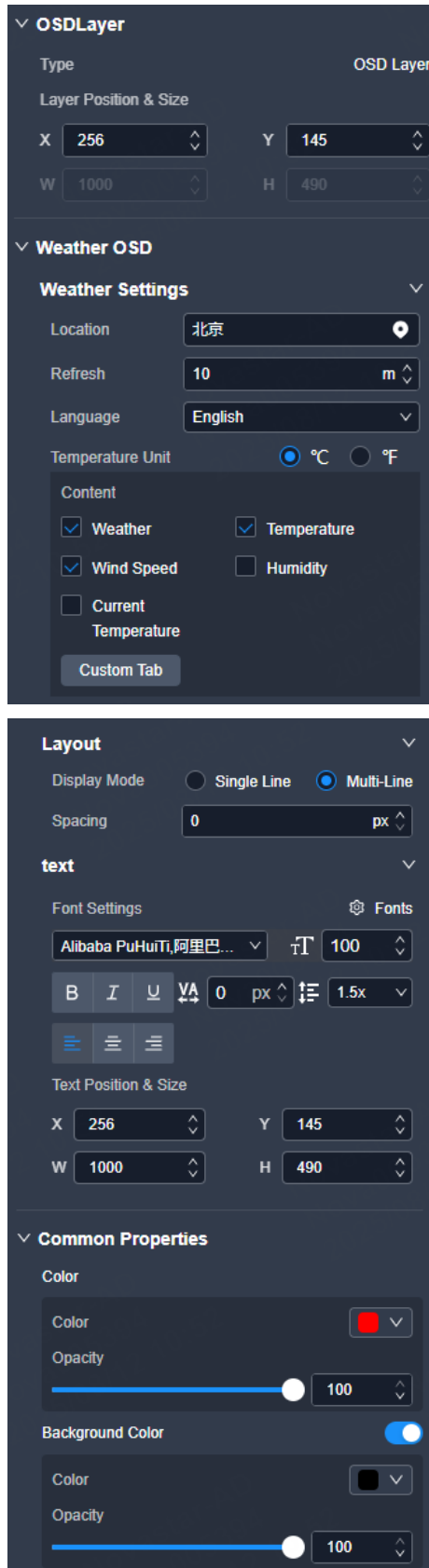
Figure 7-35 Interface example
